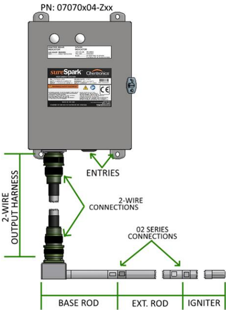
Figure 3: Ordinary area, 2-Wire LO series ignition system general arrangement.
