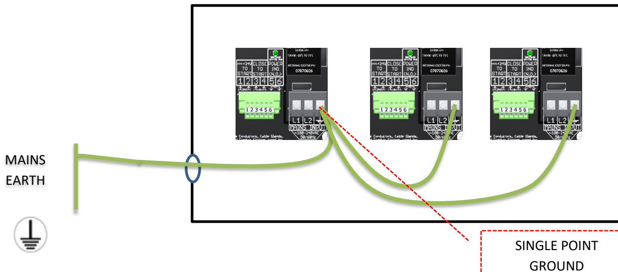
Figure 16: Earthing example (Single point ground)
