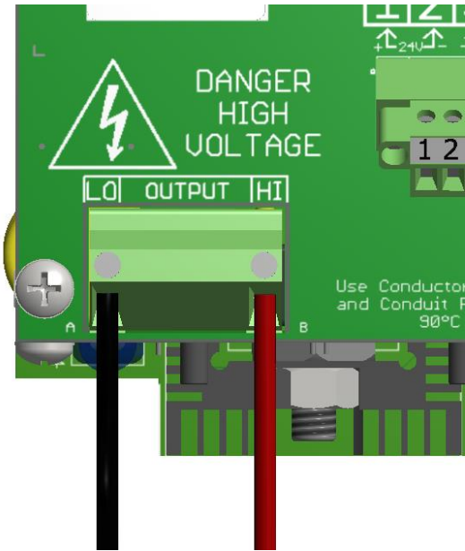
Figure 9: Correct connection of output harness wires with 1/2in NPT Male Harness.
