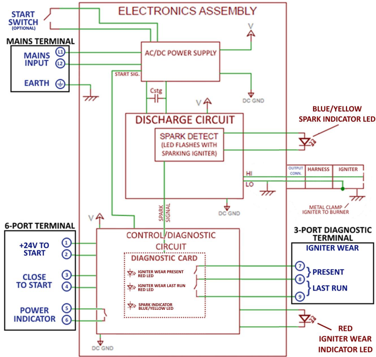
Figure 17: System schematic diagram.
