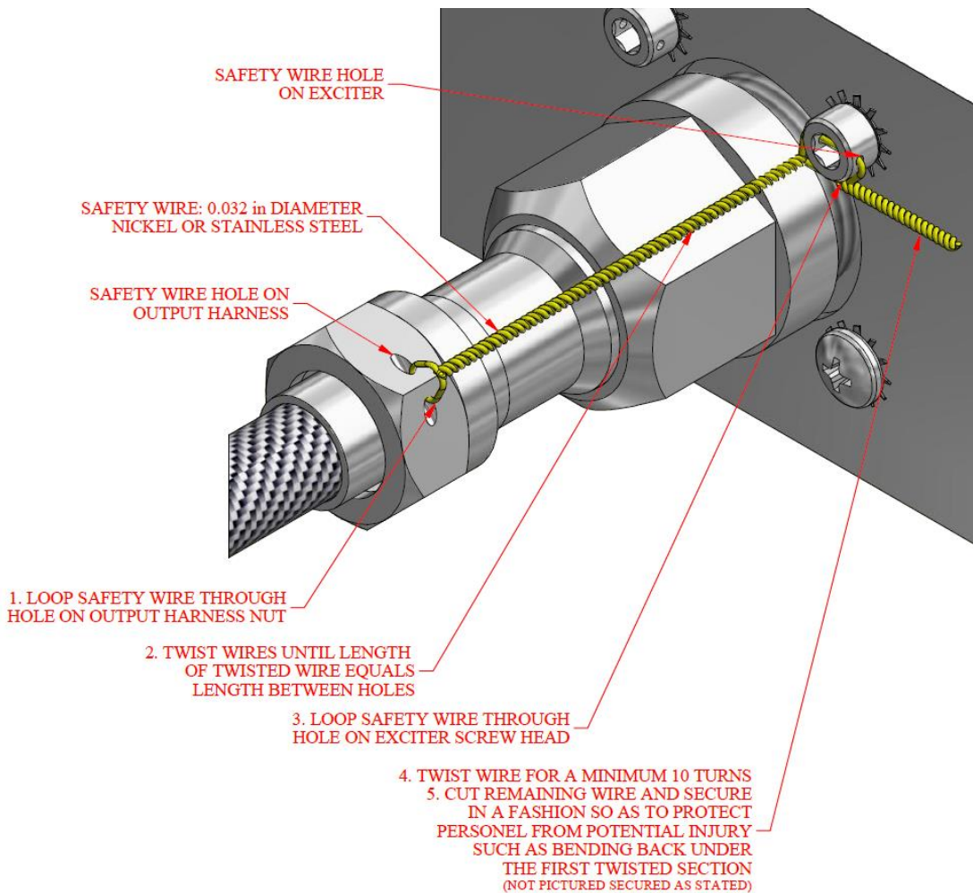
Figure 14: Safety Wire Installation – Output Harness to Exciter
