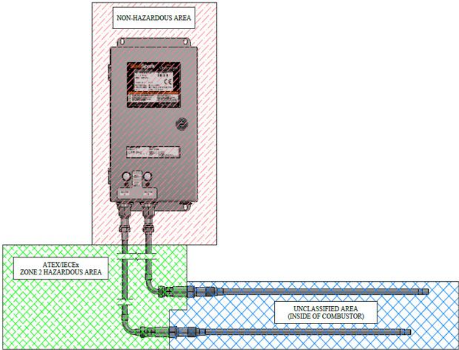
Figure 7: SureSpark™ High Energy Exciter LOTS system general arrangement. NOTE: Harnesses and igniters are sold separately.
