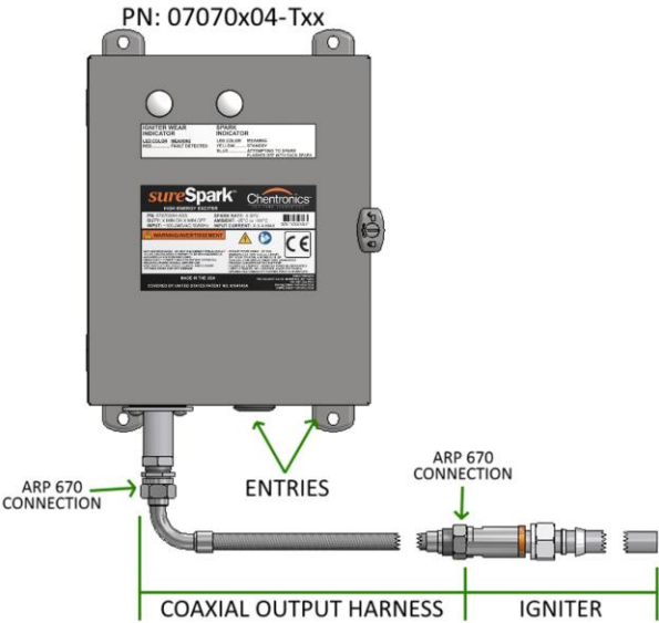
Figure 2: Ordinary area, Coaxial LO series ignition system general arrangement.
