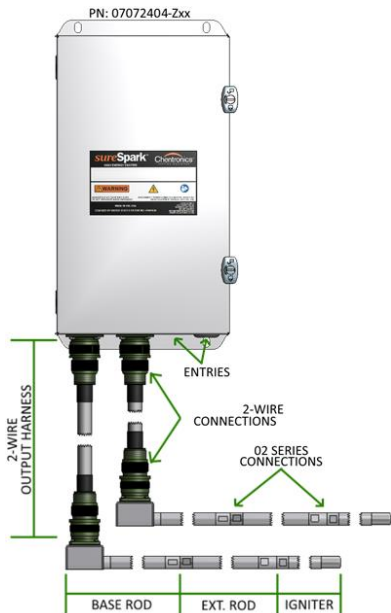
Figure 6: SureSpark™ High Energy Exciter 2-Wire Dual Output ignition system general arrangement. NOTE: Harnesses, base rods, extension rods (optional), and igniters are sold separately.
