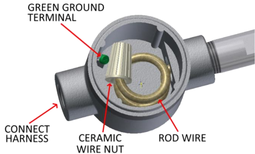
Figure 10: The case of the base rod.
