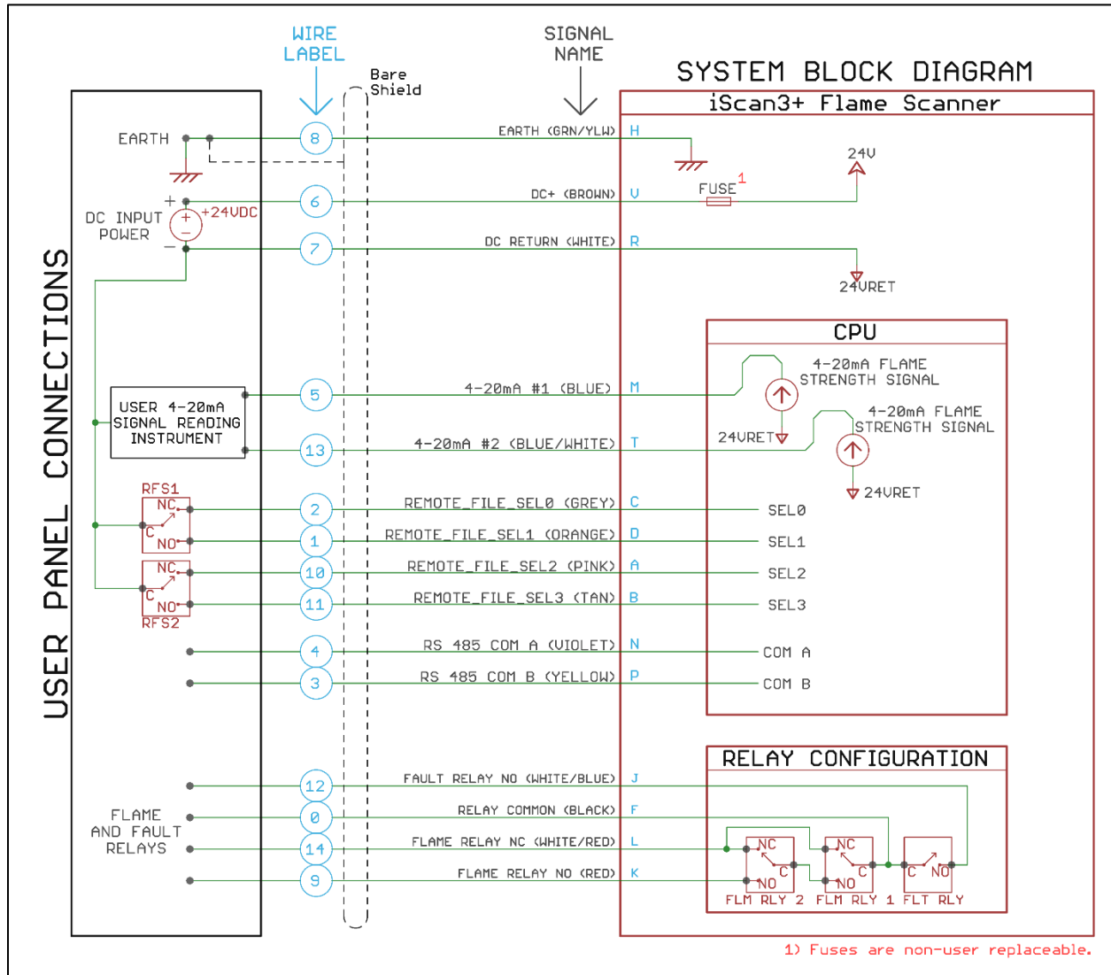
Figure 7: iScan3+ Wiring Diagram
