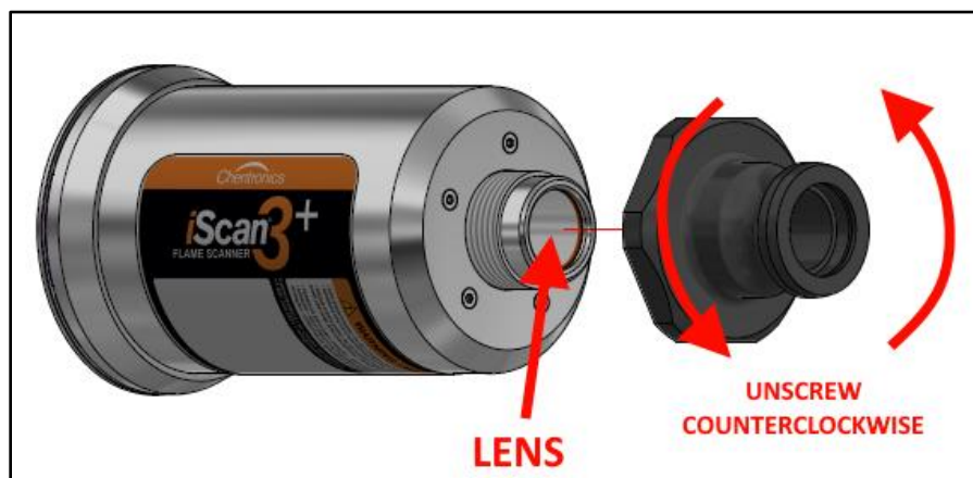
Figure 14: Lens Location
