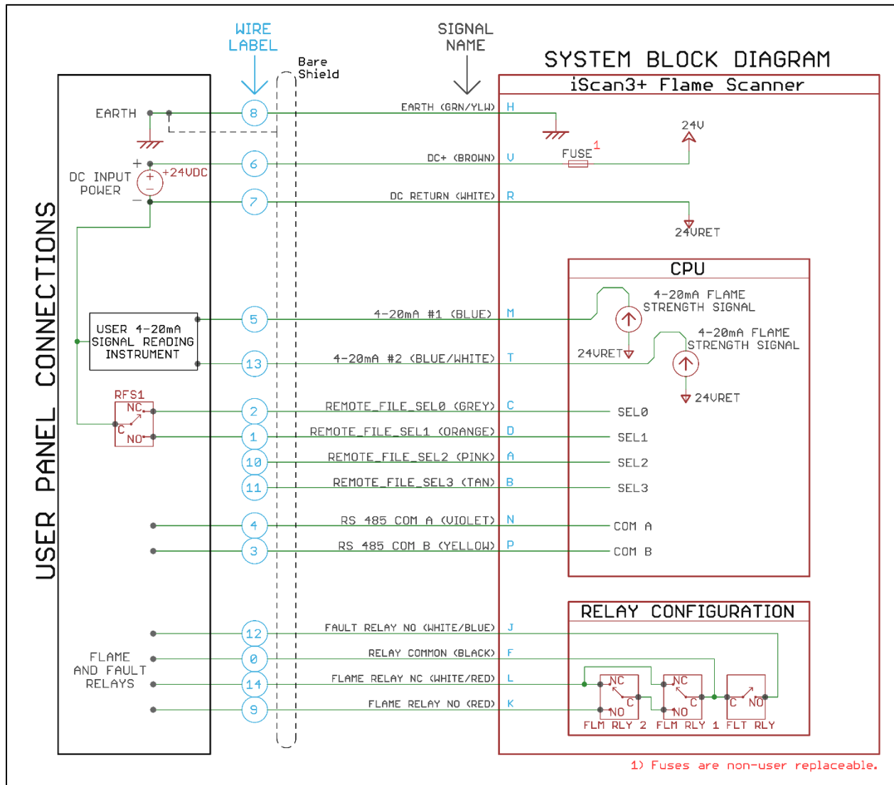
Figure 8: iScan3+ Wiring Diagram
