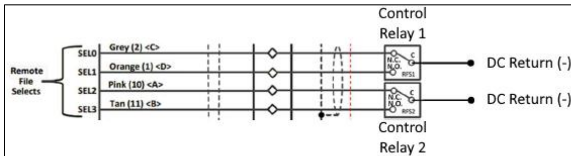
Figure 11: Schematic Diagram of Four-Wire Input
