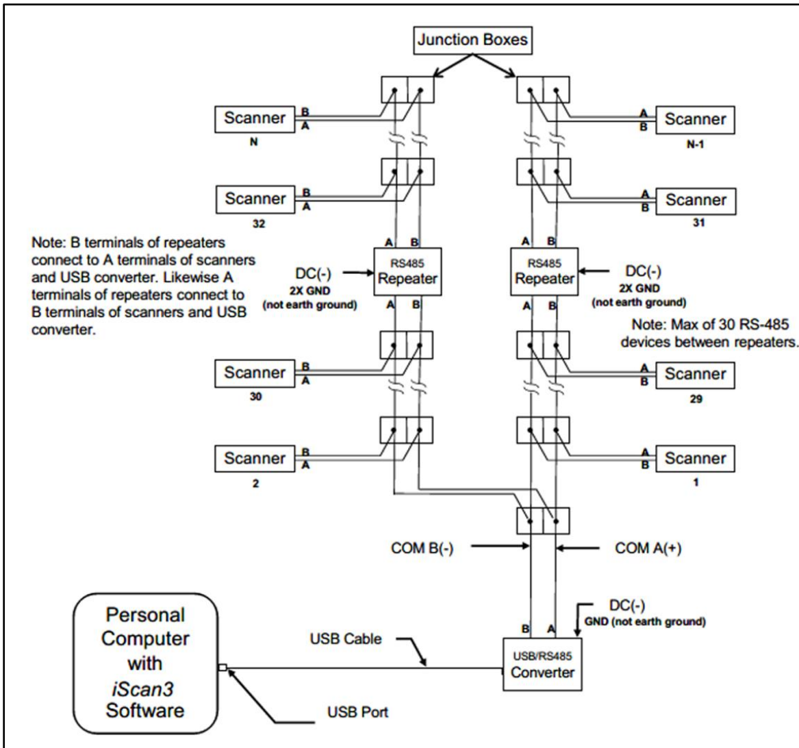
Figure 10: Split (Y Chain) Wiring Configuration
