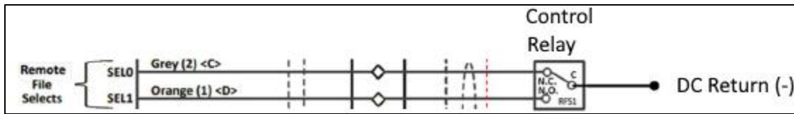
Figure 12: Schematic Diagram of Two-Wire Input
