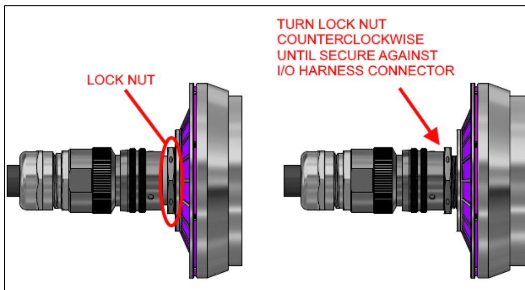
Figure 6: Division 2 Installation
